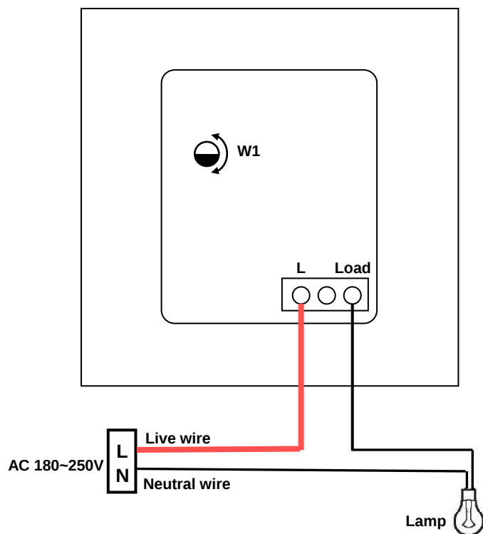
Back view
