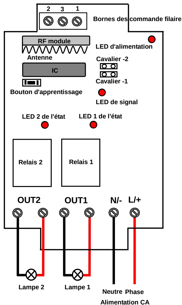
Control Lampe CA
