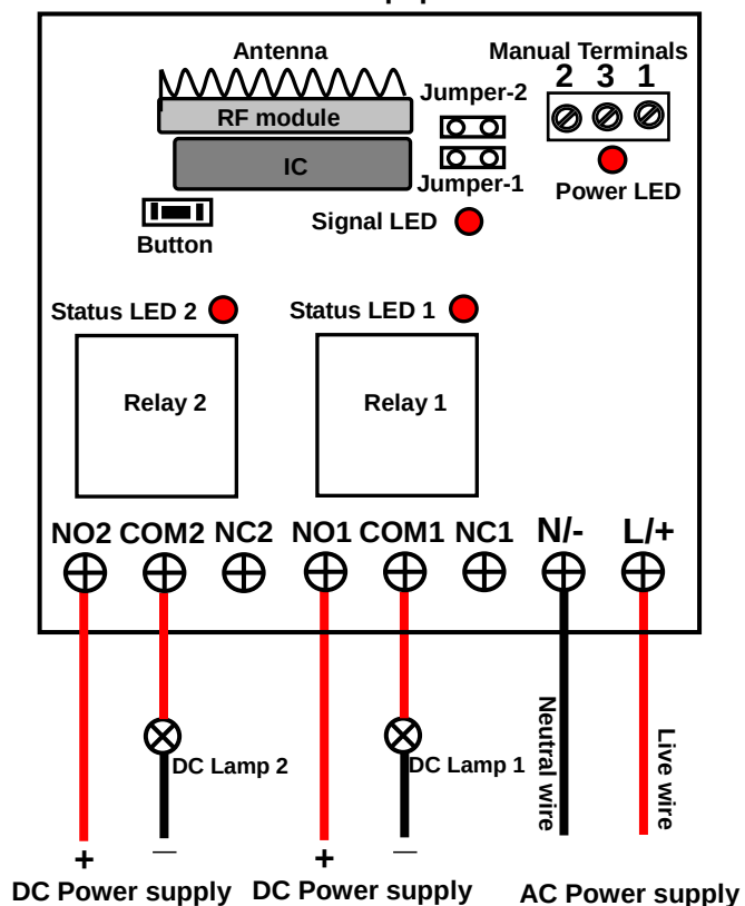
Control DC Equipment
