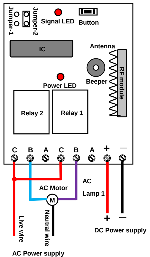
Control AC motor positive reversal direction
