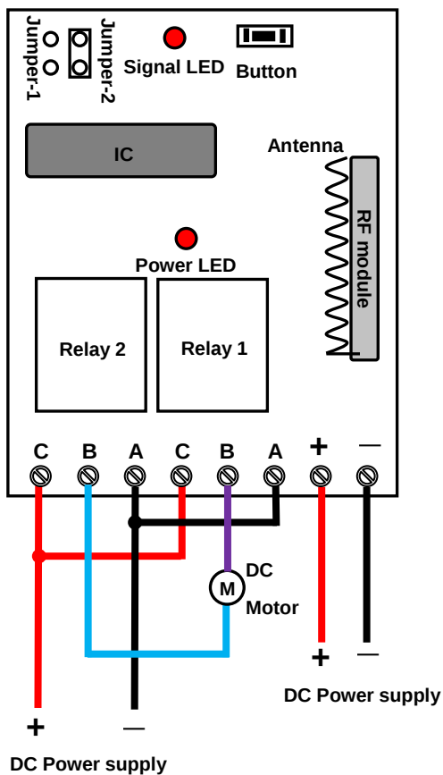
Control DC motor positive reversal direction
