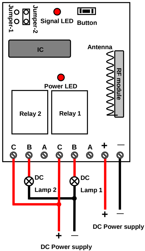
Control DC Lamp
