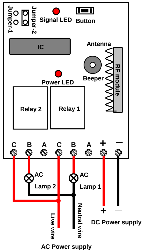
Control AC Lamp
