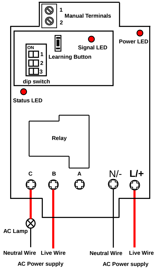
Control AC Lamp
