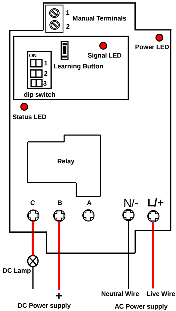
Control DC Lamp
